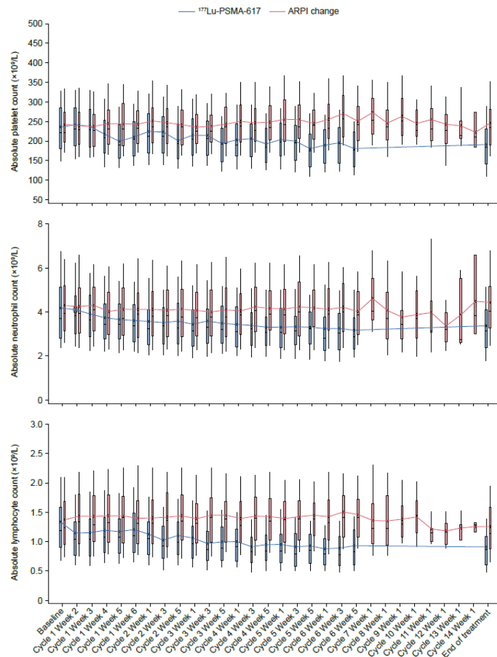
Figure S1. Change in absolute haematology parameters from baseline to end of treatment
